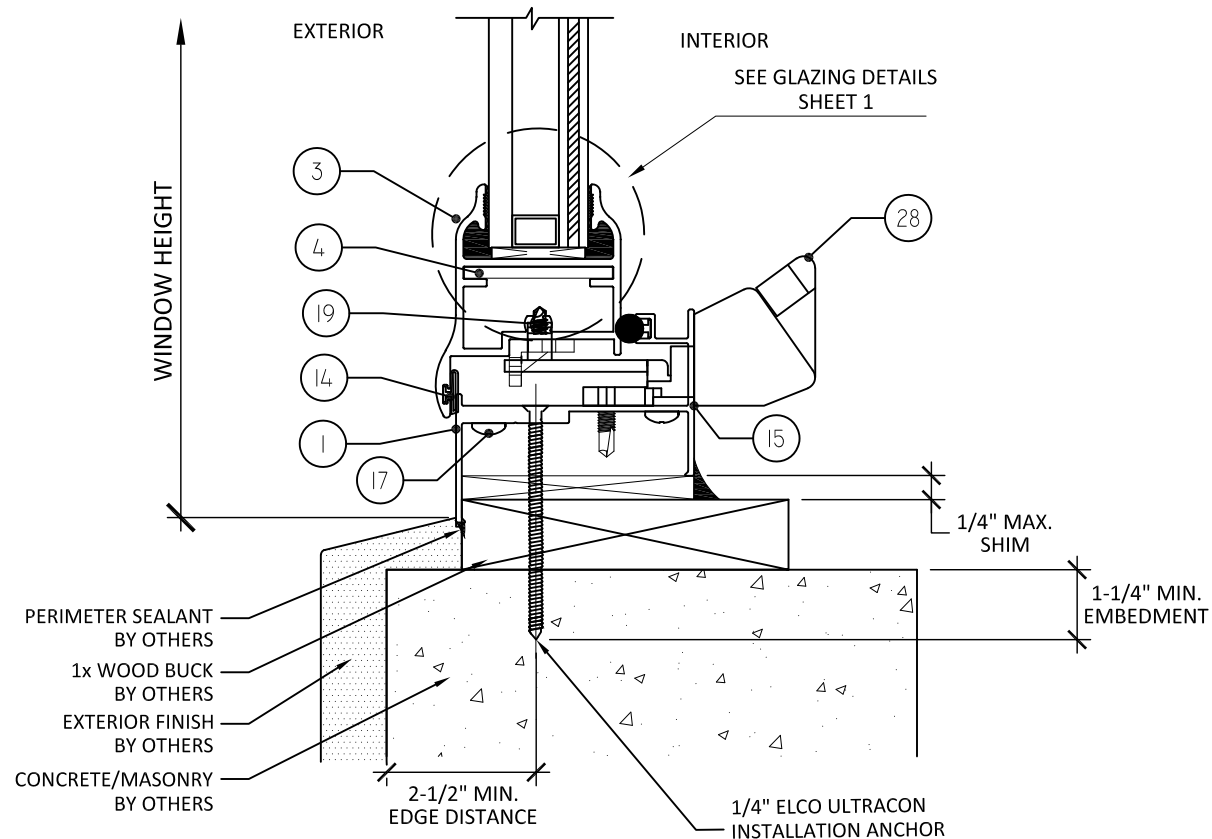
B 3 VERTICAL SECTION SILL - CONCRETE/MASONRY 1x WOOD BUCK
