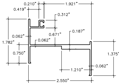
1 FRAME HEAD
