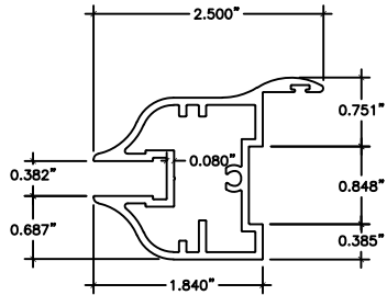
* 3B SASH PERIMETER 5/16" GLASS
