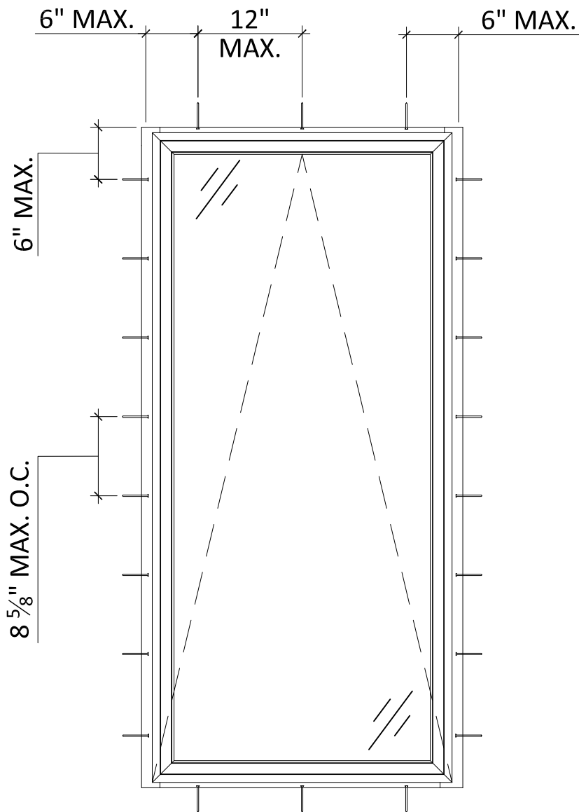
PROJECT OUT WINDOW ANCHOR LAYOUT EXTERIOR VIEW
