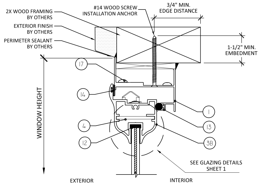
A 3 VERTICAL SECTION HEAD - 2X WOOD FRAME
