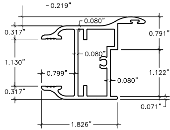
3 SASH PERIMETER
